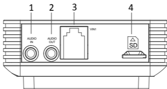
Figure 1-3 The Type II Front Panel
