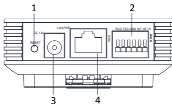
Figure 1-5 Rear Panel
