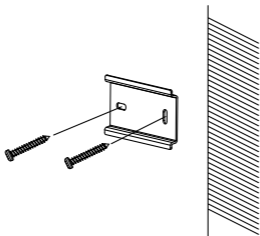
Figure 2-1 Secure the Mounting Rail
