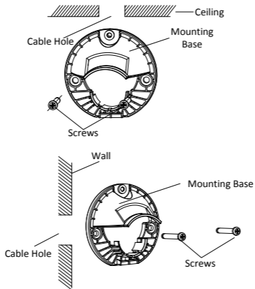
Figure 2-30 Fix the Mounting Bracket on Ceiling or on Wall
