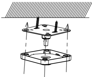
Figure 2-24 Hood the Bracket Cover
